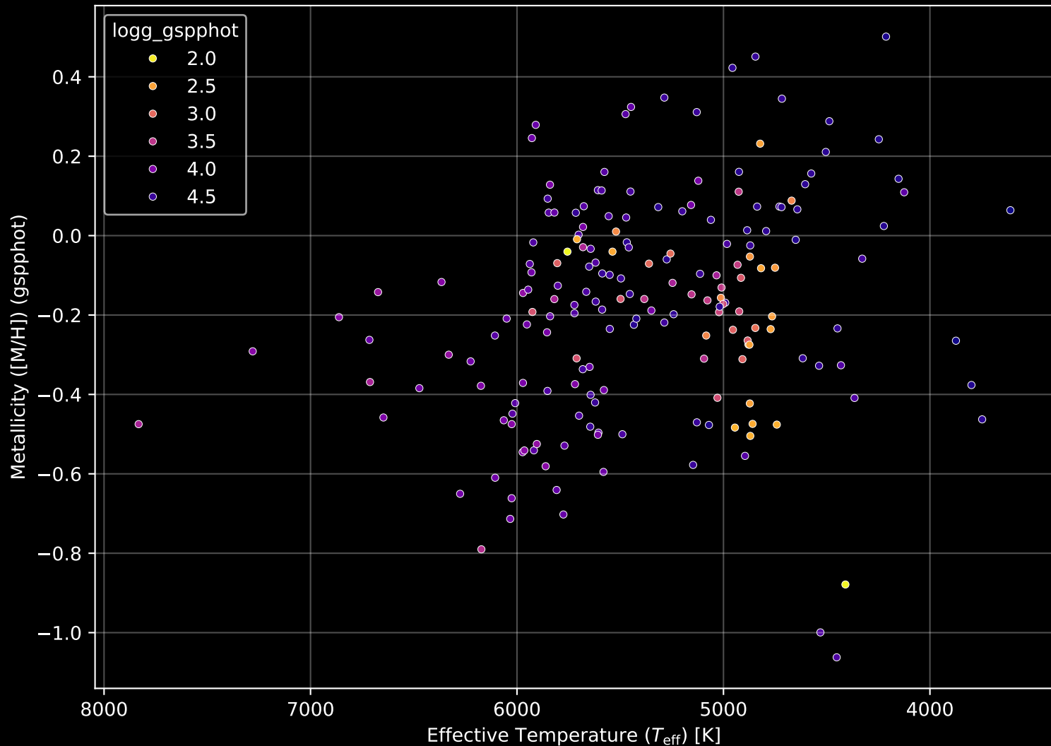
APOGEE DR17 Field: [080+59_MGA] Stellar Population Parameters (n= 188)
