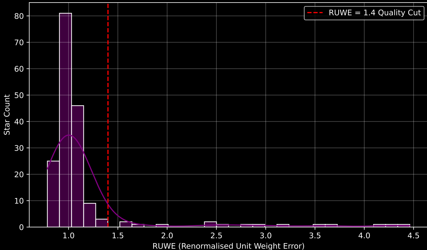
GAPOGEE DR17 Field [080+59_MGA] RUWE Distribution (n= 179)
