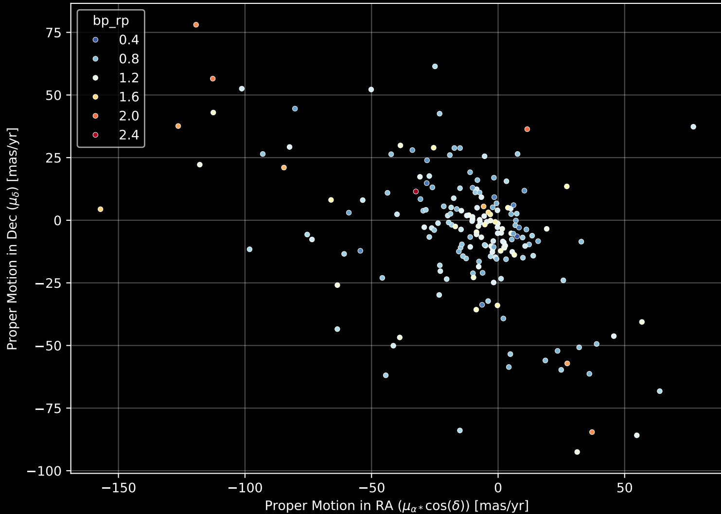
APOGEE DR17 Field: [080+59_MGA] Proper Motion Diagram (n= 188)
