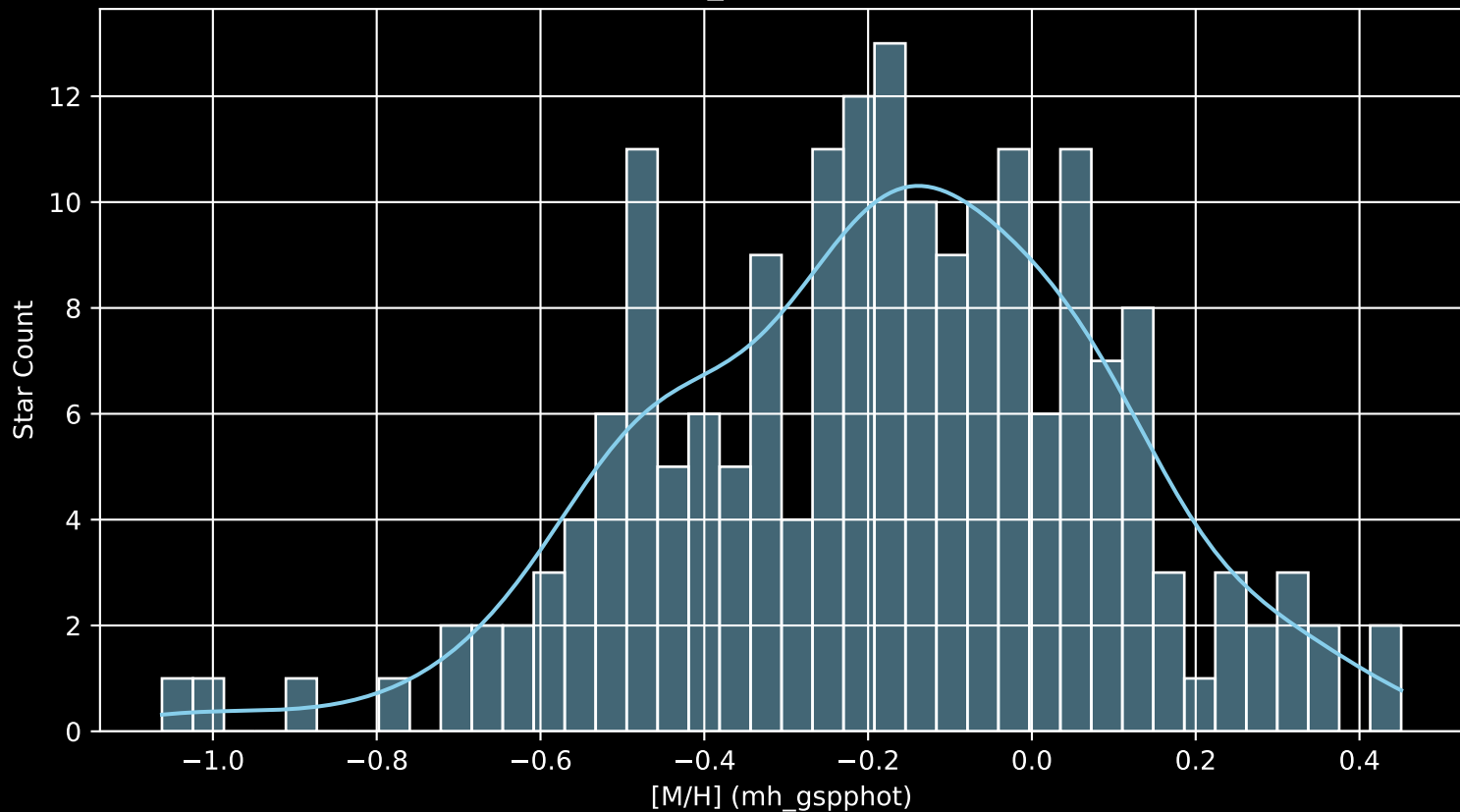
APOGEE DR17 Field: [080+59_MGA [M/H] (mh_gspphot) (n= 187)
