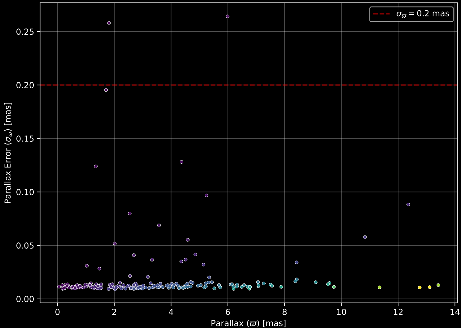
APOGEE DR17 Field: [080+59_MGA] Parallax Quality (n= 188)
