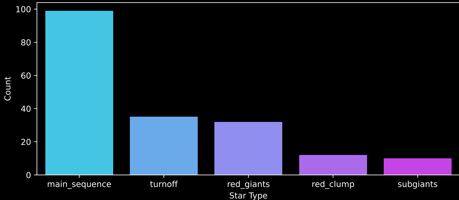
APOGEE DR17 Field: [080+59_MGA] Count plot of Star Type
